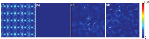
Fig. 3. (Color online) E -field distributions in a regularly arranged NW array at (a) \lambda = 899.1 nm and (b) \lambda = 916.0 nm. E -field distributions in a 48% position random NW array at (c) \lambda = 899.1 nm and (d) \lambda = 916.0 nm.
