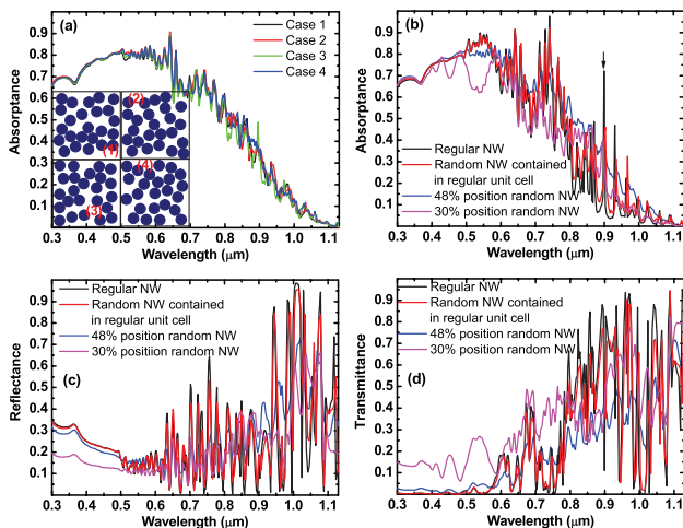
Fig. 2. (Color online) (a) Absorptance of four different 48% position random NW arrays. (b) Absorptance, (c) reflectance, and (d) transmittance of regular, random NW contained in regular unit cell, 48% position random, and 30% position random silicon NW arrays, respectively.
