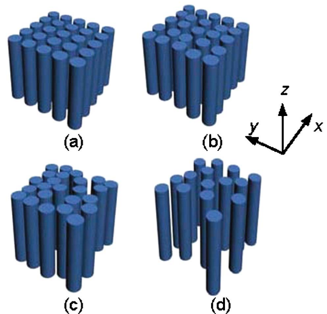
Fig. 1. (Color online) Schematics of silicon NW arrays with (a) regularly arranged square lattice, (b) random NW contained in regular unit cell used in [20], (c) 48% position random, and (d) 30% position random structure.
