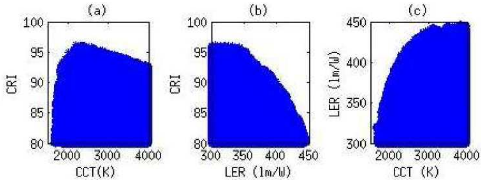
Fig. 2. Relations between (a) CRI and CCT, (b) CRI and LER, and (c) LER and CCT.
