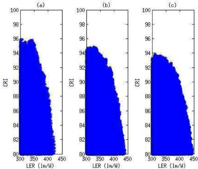
Fig. 1. CRI vs. LER dependence between (a) 2450 \text{ K} < \text{CCT} < 2550 \text{ K} , (b) 2950 \text{ K} < \text{CCT} < 3050 \text{ K} , and (c) 3450 \text{ K} < \text{CCT} < 3550 \text{ K} .
