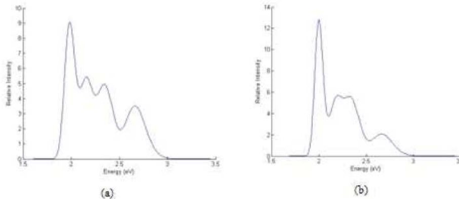
Fig. 4. The relative spectral power distribution for the average values of input parameters in the case of (a) CRI>80 and LER>300 lm/W and (b) CRI>90 and LER>380 lm/W.
