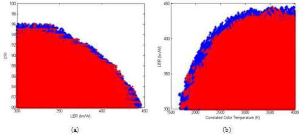
Fig. 3. (a) CRI vs. LER relationship and (b) LER vs. CCT relationship for white data points (shown in red) and near-white points (shown in blue).
